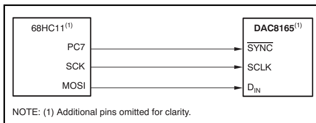
Figure 103. DAC8165 to 68HC11 Interface
