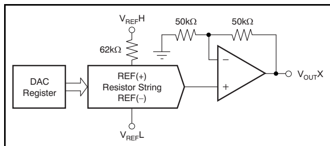
Figure 92. DAC8165 Architecture
